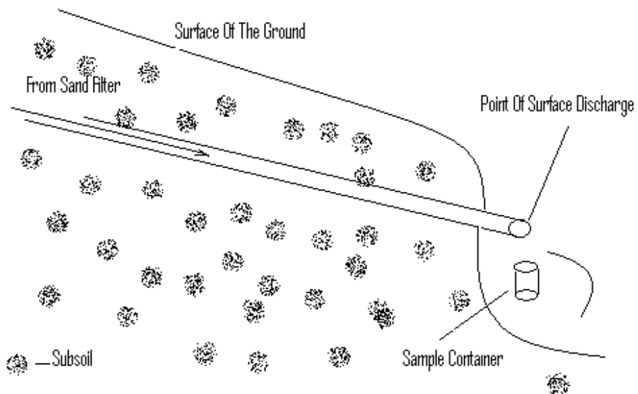
Diagram B Example Wastewater Sampling Port For Surface Discharging System
